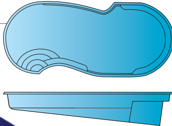
IOWA 15'6" wide x 35' long 3'7" to 5'9" deep
